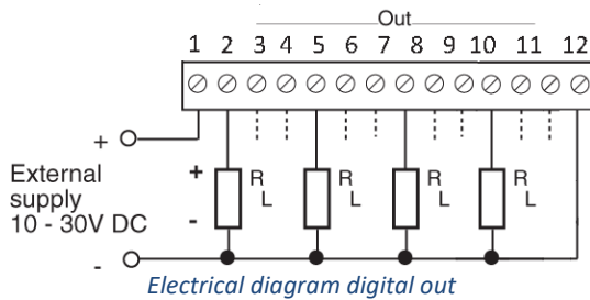
Electrical diagram digital out
