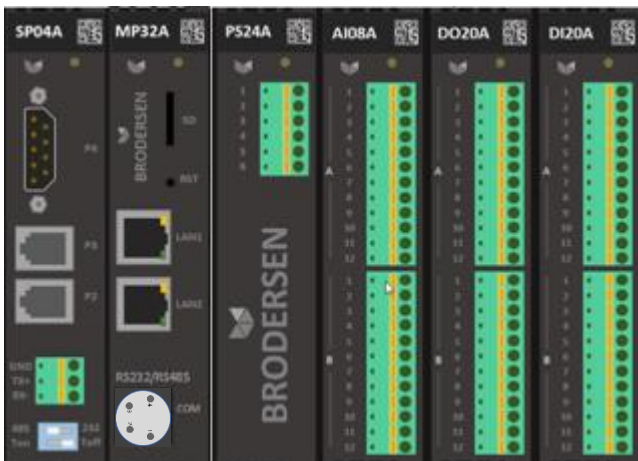
Figure 6: MP32A Rev. C hardware interface with I/O
