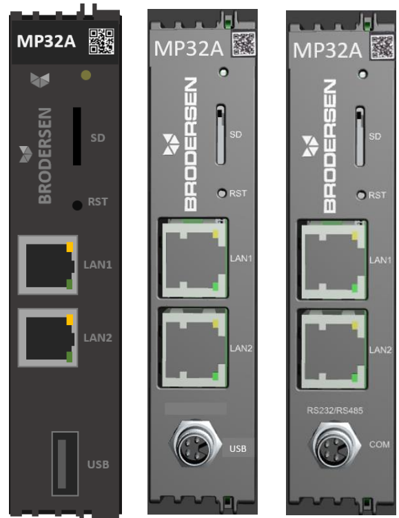
Figure 1: MP32A Rev. A, B & C front view
