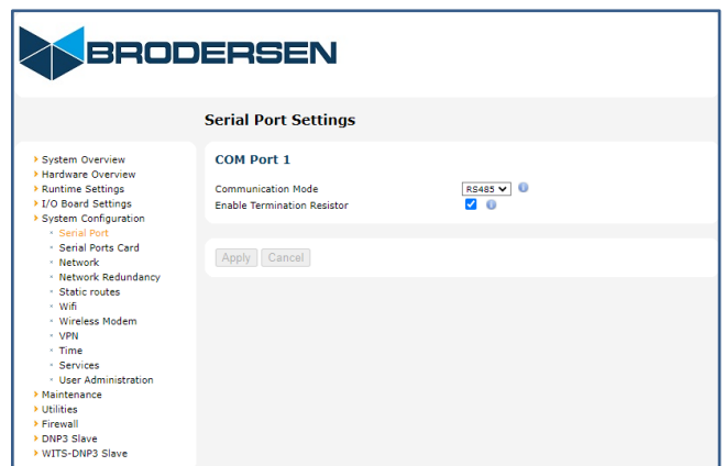
Figure 7: By default, serial port web configuration
