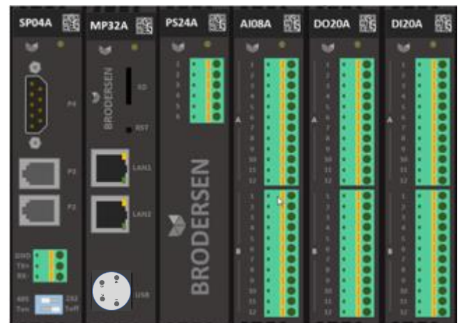
Figure 5: MP32A Rev. B hardware interface with I/O
