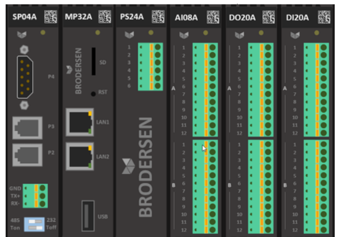
Figure 4: MP32A Rev. A hardware interface with I/O
