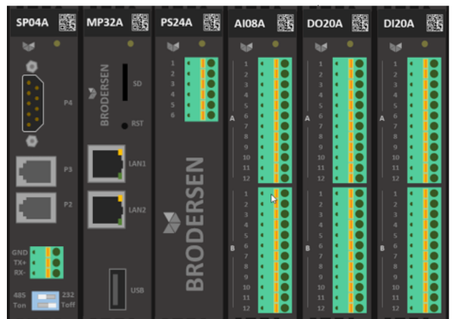
Figure 3: MP32A hardware interface with I/O
